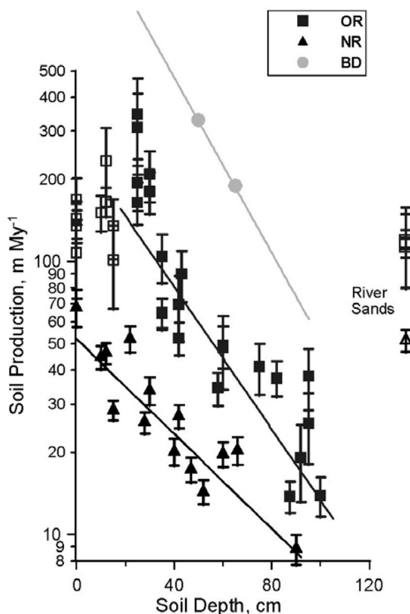
Figure 9. The soil production functions for three sites. These data bracket the entire data set of 7 sites reported in Heimsath [1999]. The Nunnock River area (NR), southeastern Australia [Heimsath et al., 2000], had the lowest production rate for a given soil thickness, with \epsilon_0 = 53 m/my, \alpha = -0.02 (1/m). Sites at Point Reyes, California [Heimsath 1999], \epsilon_0 = 81 m/my, \alpha = -0.016 (1/m) and Frogs Hollow, southeastern Australia [Heimsath et al., 2001b], \epsilon_0 = 141 , \alpha = -0.042 , lie between the Nunnock River and Oregon Coast Range [Heimsath et al. 2001a], \epsilon = 268 , \alpha = -0.03 . Data from the San Gabriel Mountains were similar to the Oregon Coast Range, i.e. \epsilon = 318 , \alpha = -0.038 . Oregon (OR) production rates for shallow samples and exposed bedrock samples (open squares) were not used in the regression. See text for further discussion. The soil production rates at all sites except Black Diamond Mine (BD) were determined by using concentrations of in situ produced cosmogenic nuclides as described in Heimsath et al. [1999]. The two values at BD were derived from garden variety ^{10}\text{Be} in soils [McKean et al., 1993] and suggest \epsilon = 2078 , \alpha = -0.037 .
