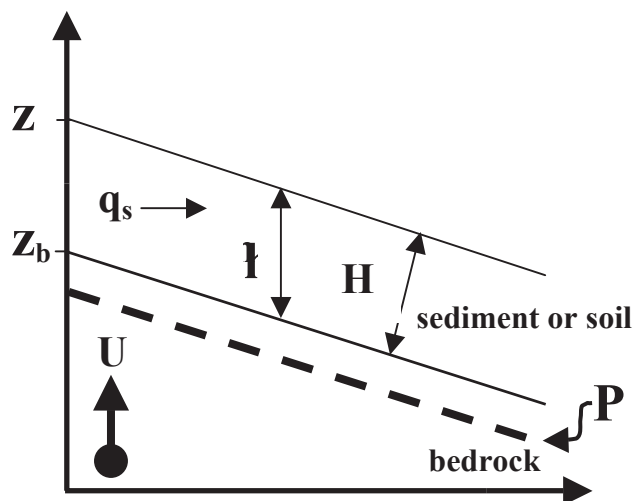
Figure 5. Cartoon illustrating terms in conservation of mass expression (equation 1) for a soil-mantled hillslope or sediment-mantled channel with a ground surface elevation of z . The soil or sediment thickness is h , and uplift, U , is shown as positive upward. Dashed line below soil-bedrock interface illustrates the depth of bedrock converted to soil over a given time period (e.g. soil production rate, P ). The sediment transport per unit hillslope width is q_s . The normal depth, H , and the elevation of the soil-bedrock boundary, z_b , used in equation (11) are also shown.
