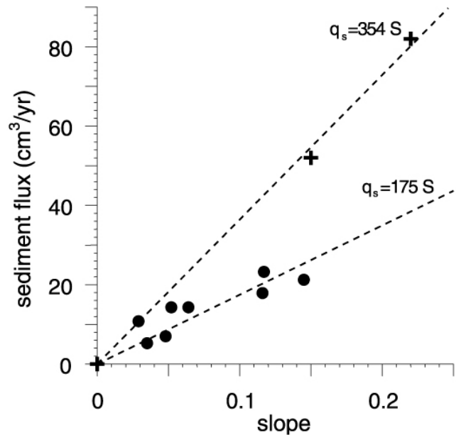
Figure 6. Plot of slope versus soil flux rate for sites in a clay-rich soil in coastal California (crosses; from McKean et al., 1993 ) and an alpine hillslope in the Wind River Range, Wyoming (infilled circles; from Small et al., 1999 ). Data from both sites (acquired using cosmogenic radionuclides)
