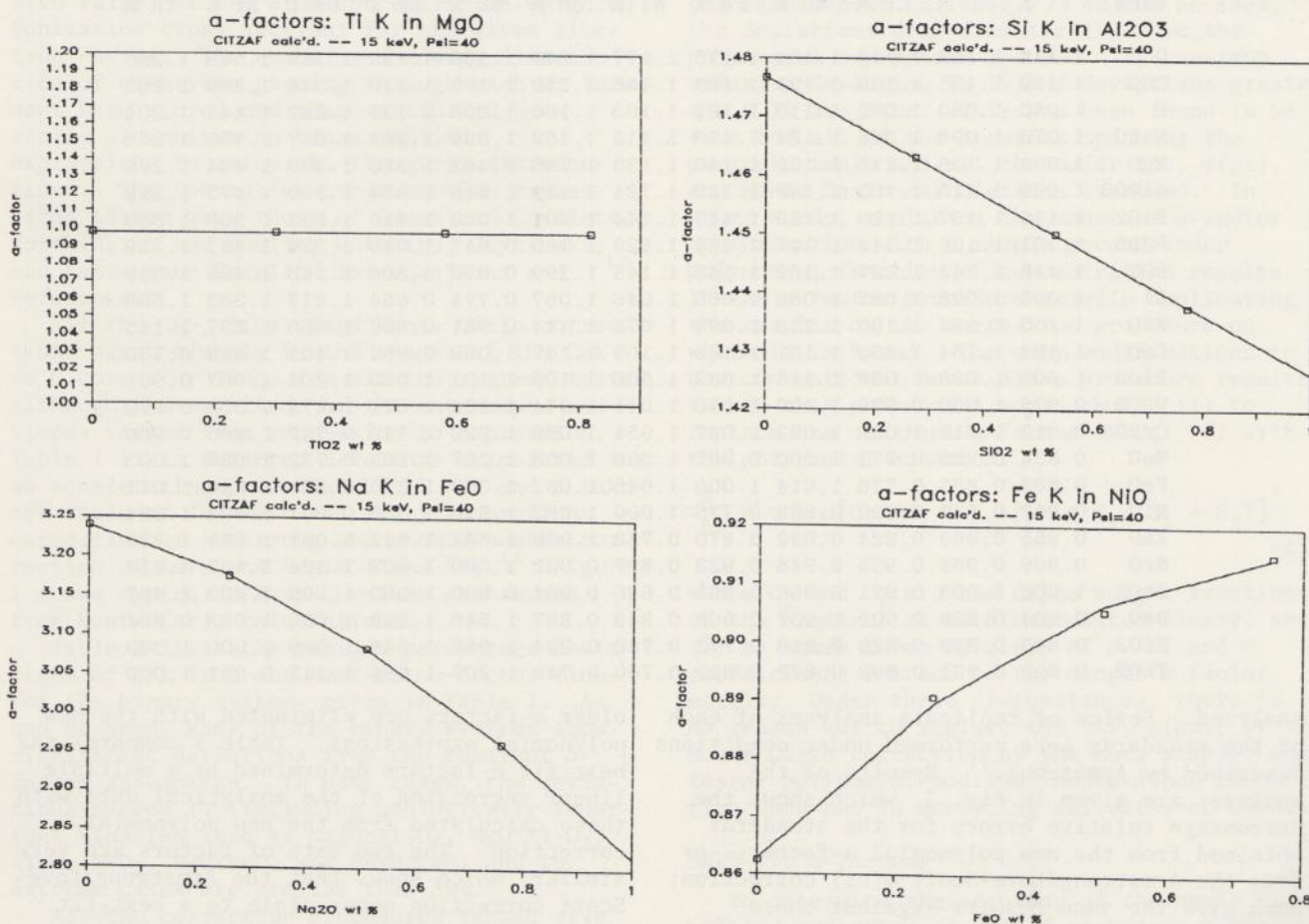
FIG. 2.--Plots of calculated \alpha -factor vs concentration, in oxide weight fraction, for (a) Ti K \alpha in TiO 2 :MgO, (b) Si K \alpha in SiO 2 :Al 2 O 3 , (c) Na K \alpha in Na 2 O:FeO, (d) Fe K \alpha in FeO:NiO.
