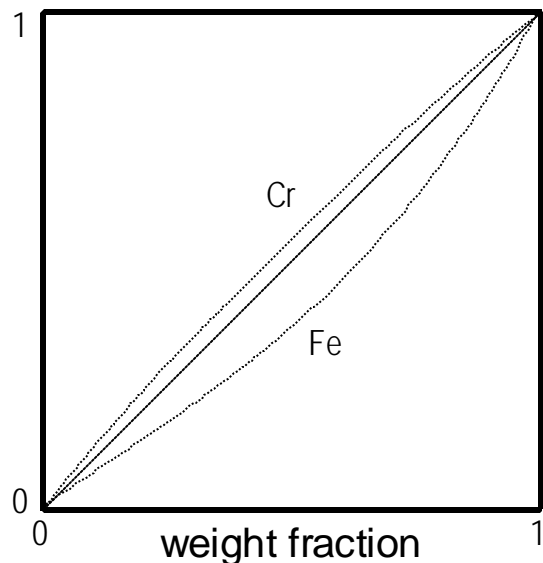
Figure 3-12 The fluorescence of Cr K\alpha x-rays due to absorption of Fe K.
