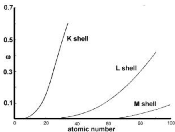
Figure 3-6 Fluorescence yield, \omega , for the K, L and M families of x-rays as a function of atomic number (Goldstein et al., 1984).
