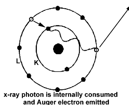
Figure 3-5 Schematic diagram illustrating the internal consumption of an x-ray photon and production of an Auger electron.
