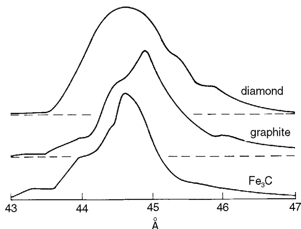
Figure 3-9 Variation in the area normalized peak shape and location for the carbon K line as measured from
