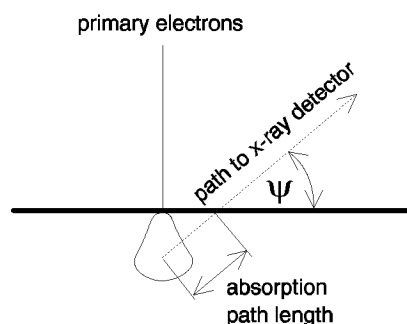
Figure 3-10 The path length for x-ray absorption from the interaction area through the sample line-of-sight to the detector. The angle between the planar surface and
