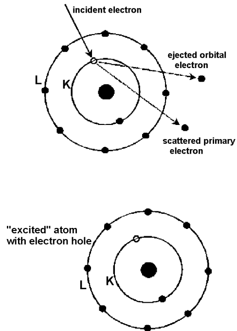
Figure 3-1 Schematic diagram illustrating the ejection of an K-shell electron and production of an unstable electron hole
