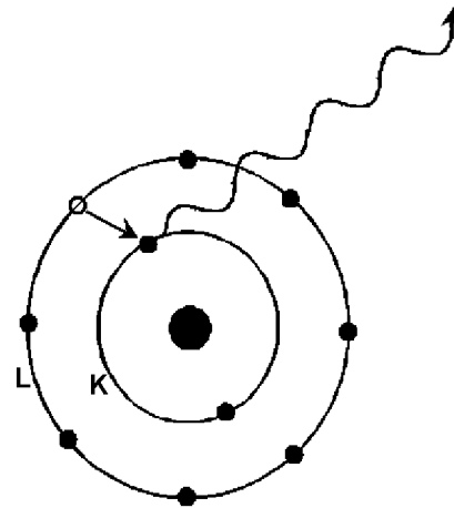
electron hole is filled and x-ray photon generated
