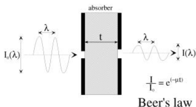
Figure 3-11 Beer's law.
