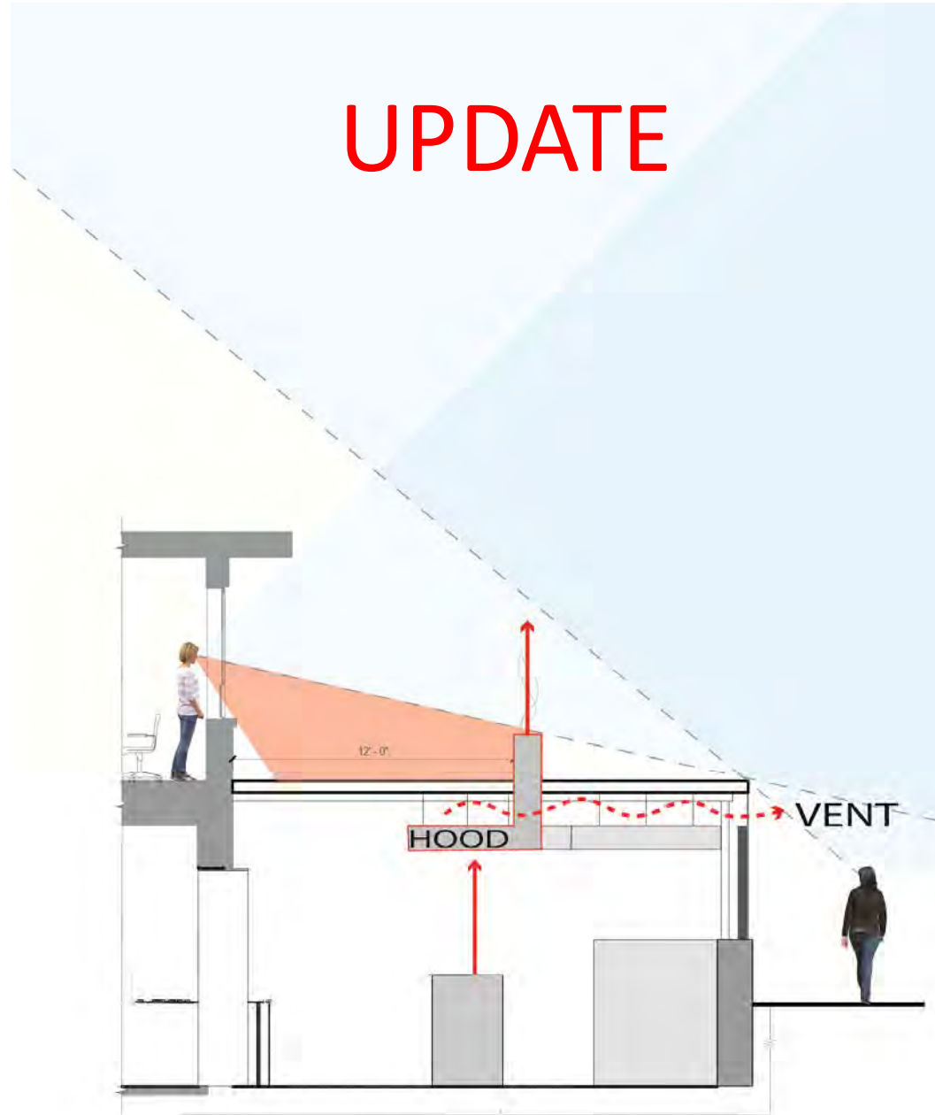
OUTDOOR CRAFT CENTER ENCLOSURE - VENTING SECTION
