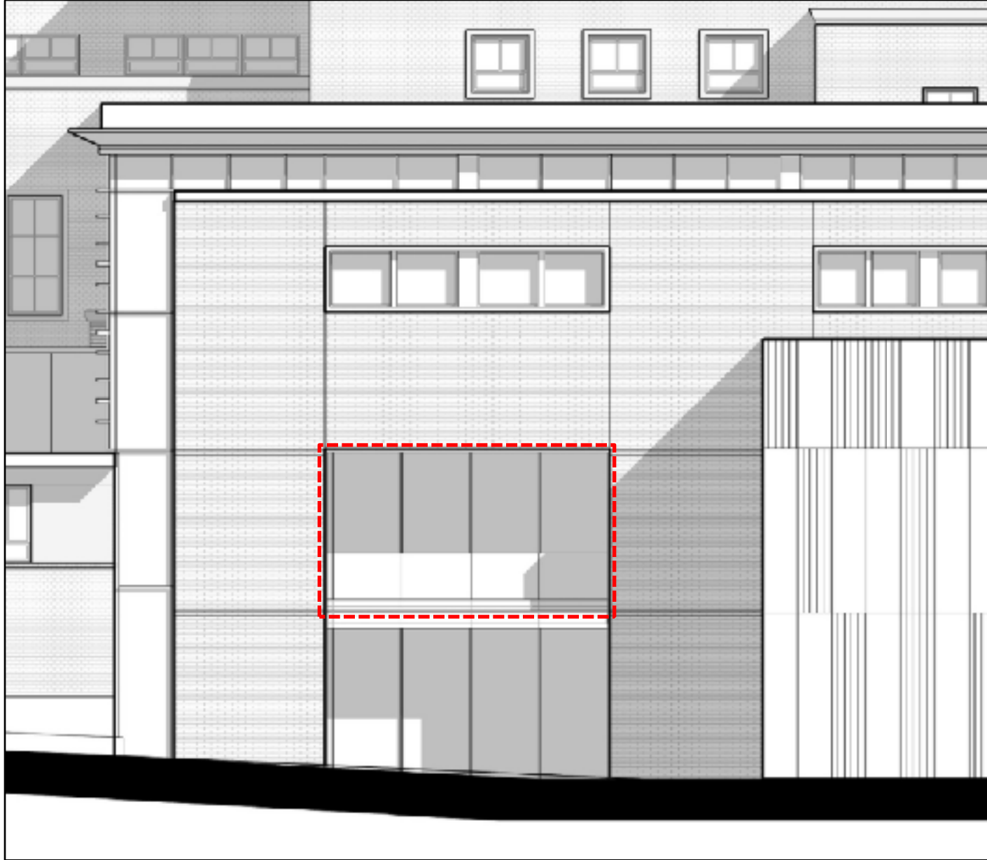
EAST ELEVATION – SEATING BALCONY
