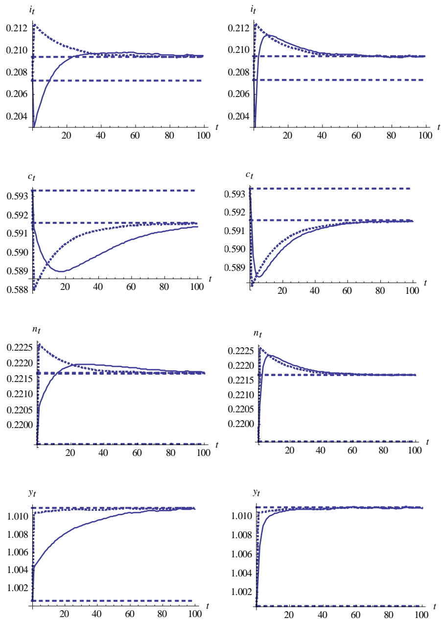
Figure 4: Impact of gain parameter. The left hand side illustrates the dynamics with a smaller gain of 0.01 and the right hand side the dynamics with a larger gain of 0.08. Solid lines show learning dynamics and dashed line the RE dynamics. Mean paths over 20,000 replications.
