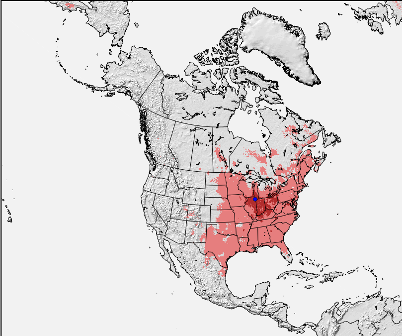
Analogue of Present Climate
