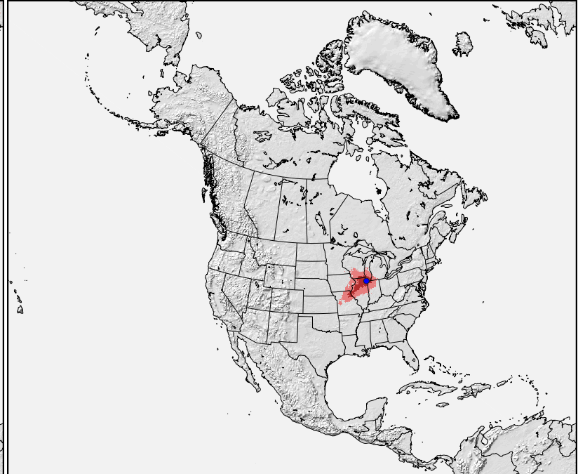
Analogue of Future Climate
