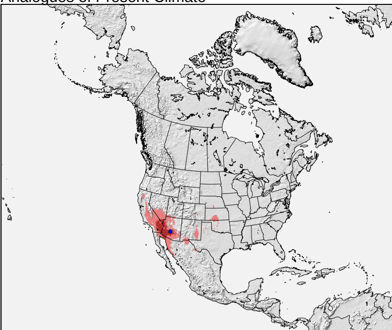
Analogues of Present Climate
