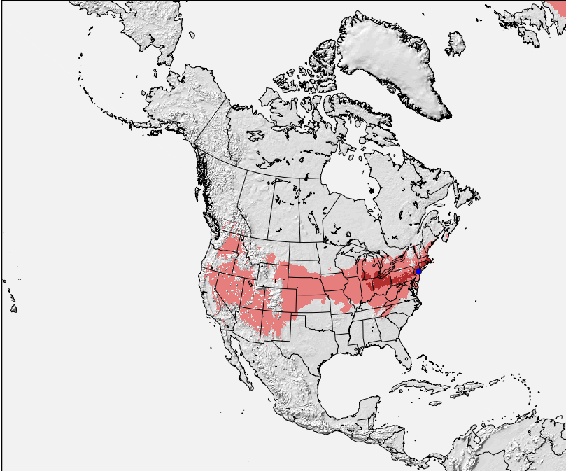
Future Locations of Present Climate
