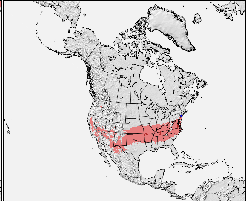
Present Locations of Future Climate
