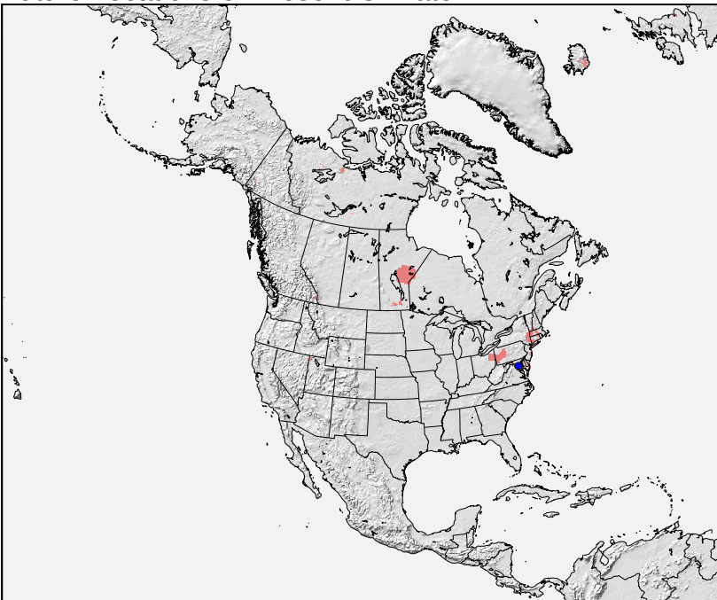
Future Locations of Present Climate
