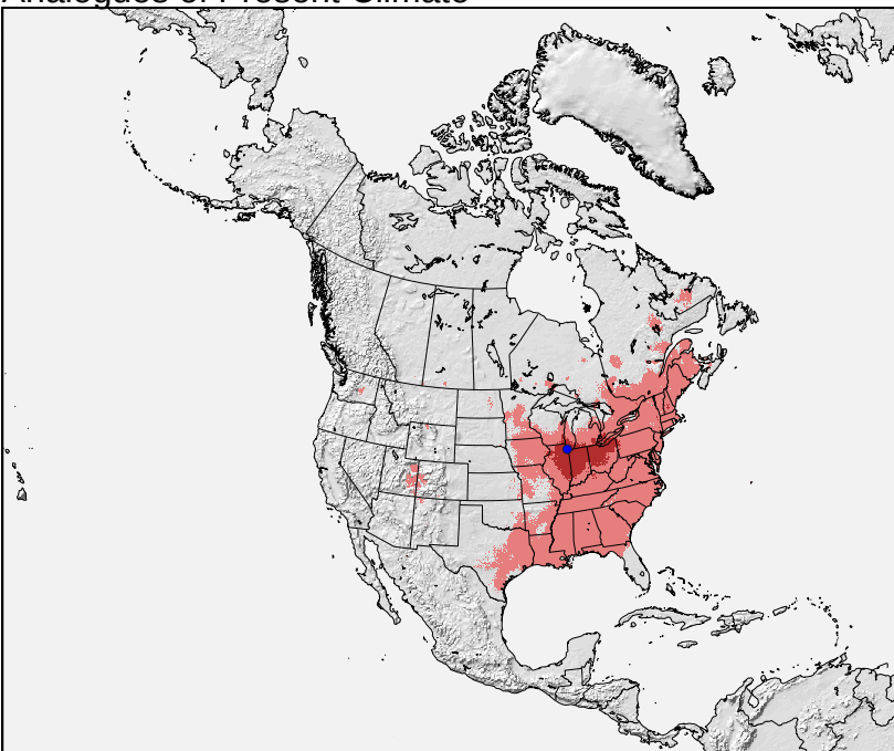
Analogue of Present Climate
