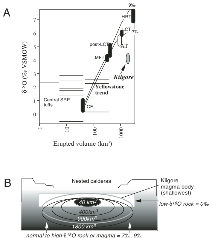
Figure 3. Origin of large-volume low \delta^{18}\text{O} magmas in caldera settings. A: \delta^{18}\text{O} values of bulk magma plotted against its eruptive volume, where low \delta^{18}\text{O} , 0‰ hydrothermally altered rock or magma are bulk mixtures between normal \delta^{18}\text{O} magma and 7‰ (lower curve) and 9‰ (upper curve) lower crustal magma, respectively. Mixing lines are drawn assuming ellipsoidal geometry of magma chambers from panel B, in which low \delta^{18}\text{O} rocks are confined to the intracaldera block. In A, Yellowstone magmas define a trend of mixing between most \delta^{18}\text{O} depleted, ~0‰ Canyon flow (CF) rhyolites of small 40 km 3 volume and normal \delta^{18}\text{O} , 8‰ Huckleberry Ridge tuff (HRT)–type magma. The most \delta^{18}\text{O} depleted CF rhyolite from Yellowstone represents 100% remelting of the low \delta^{18}\text{O} hydrothermally altered rocks, while HRT-type magma that erupted at the inception of volcanism at Yellowstone represents the lower crust–derived normal \delta^{18}\text{O} component. Intermediate \delta^{18}\text{O} magmas such as Lava Creek tuff (LCT), Mesa Falls tuff (MFT), and post-LCT 0.2 Ma Yellowstone rhyolites are plotted vs. their respective eruptive volumes and plot on the overall Yellowstone mixing (or low \delta^{18}\text{O} diluting) trend. The voluminous 1000 km 3 low \delta^{18}\text{O} Ammonia Tanks tuff (AT) of Timber Mountain Caldera complex, Nevada (Bindeman et al., 2006), also plots on this mixing trend. Thin lines are central Snake River Plain (SRP) low \delta^{18}\text{O} units (Boroughs et al., 2005) with poorly defined volumes plot variably. VSMOW—Vienna standard mean ocean water. B: Conceptual model of mixing of low \delta^{18}\text{O} carapace melt with normal \delta^{18}\text{O} magma from below in caldera settings. The low \delta^{18}\text{O} end member is diluted over progressively larger magma volumes when vertical and horizontal sizes of the magma chamber increase. Bulk \delta^{18}\text{O} of final magma results from volumetric contributions from the low \delta^{18}\text{O} cap and the normal \delta^{18}\text{O} magma chamber as indicated by the ellipsoids. Based on these constraints, the more voluminous Kilgore magma body taps a greater proportion (~40%) of low \delta^{18}\text{O} carapace compared to Yellowstone. Alternatively, if \delta^{18}\text{O} depletion in the carapace is greater compared to Yellowstone, smaller proportions of low \delta^{18}\text{O} melts will suffice.
