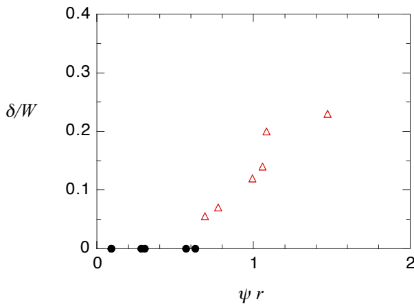
Figure 3. Shear region width \delta/W as a function of \psi r , for small aspect ratios ( r < 0.25 ). The experiments had a bottom slope \theta = 3.5^\circ , and consisted of either flow with a central solid crust bounded by shear layers ( \Delta ) or tube flow with \delta = 0 ( \bullet ).
