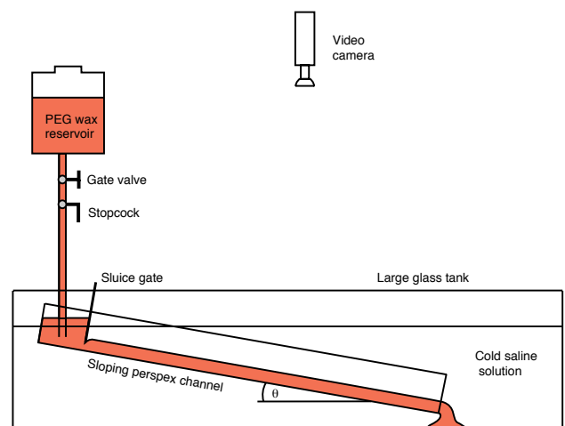
Figure 1. Diagram of the experimental apparatus.
