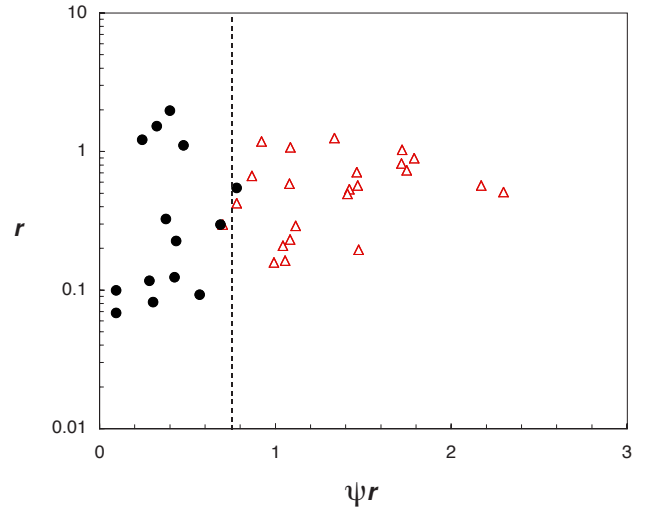
Figure 4. Classification of flows under all experimental conditions into either tube flow with a fixed solidified roof ( \bullet ) or flows with a mobile solid crust confined to a central strip ( \Delta ). Runs with bottom slopes of both \theta = 1.6^\circ and \theta = 3.5^\circ are included. The boundary between the two flow regimes is given approximately by \psi r = 0.75 (shown as a vertical dashed line).
