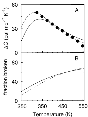
Figure 4. Least-squares fit of the two-state transfer heat capacity to the experimental data for Argon, comparing the best-fit curve (dashed line, \Delta H_{\text{shell}} = 2.4 kcal mol -1 and \Delta S_{\text{shell}}/k = 3.2 ) with a fit having the f_{\text{bulk}} and f_{\text{shell}} curves constrained to cross at 450 K (177 °C) (solid line, \Delta H_{\text{shell}} = 2.4 kcal mol -1 and \Delta S_{\text{shell}}/k = 3.0 ). (B) f_{\text{bulk}} (solid line) and f_{\text{shell}} (dotted line) corresponding to the solid line in part A.
