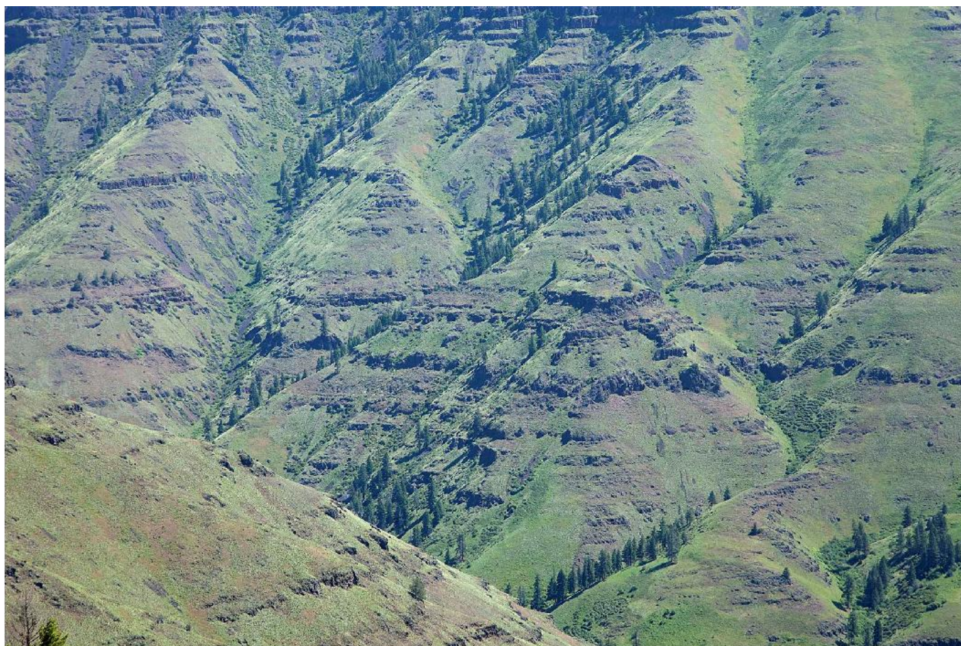
Grande Ronde basalt flows in the Joseph Creek Canyon, Oregon. The Grande Ronde Basalt is part of the Miocene Columbia River Basalt Group. Photo by Marli Miller
