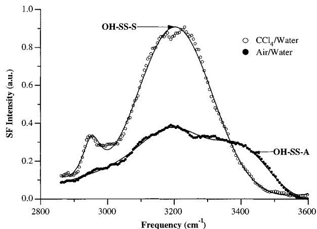
Figure 1. VSFG spectra under S-sfg, S-vis, and P-ir polarization conditions from the neat \text{CCl}_4 /water (open circles) and air/water (filled circles) interfaces. Solid lines are a fit to the data using eqs 1 and 2.
