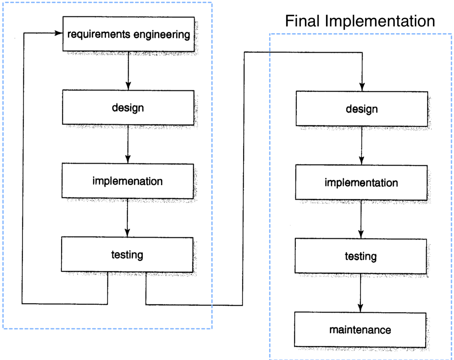
Figure 3.3 Prototyping as a tool for requirements engineering
