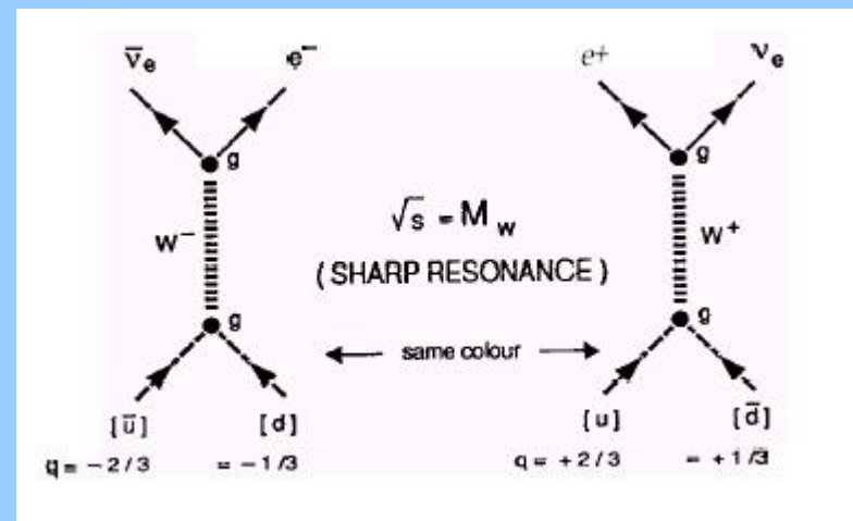
q anti- q annihilation to W^\pm
