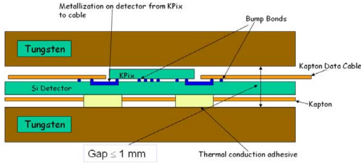
Figure 1. Schematic of the readout gap. With power cycling of the readout chip, the heat load of the KPiX readout chip can be handled by passive conduction through the tungsten.
