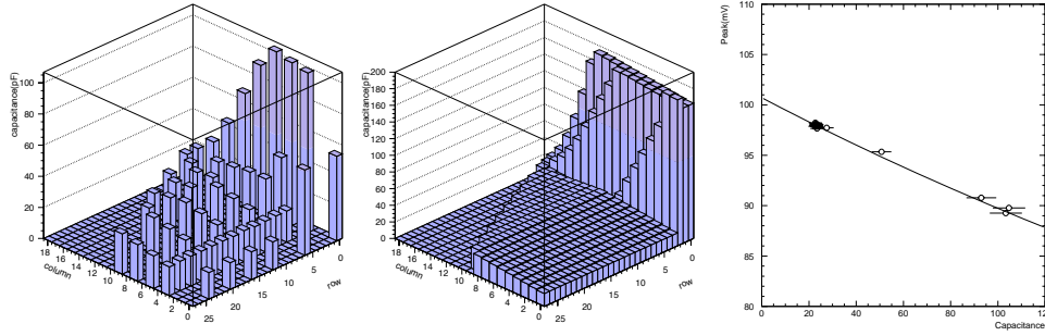
Figure 2. Summary of capacitance measurements as a function of pixel position on the detector. Figure on left is current measurements, where the high capacitance of pixels at small row number is due to large number of traces in that region. Center figure is the expected capacitance in a 1024 pixel version of the sensor. Figure on right is the measured position of ^{241}\text{Am} peak signal versus total pixel capacitance.
