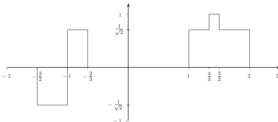
FIGURE 1. Graph of \hat{\psi} .
