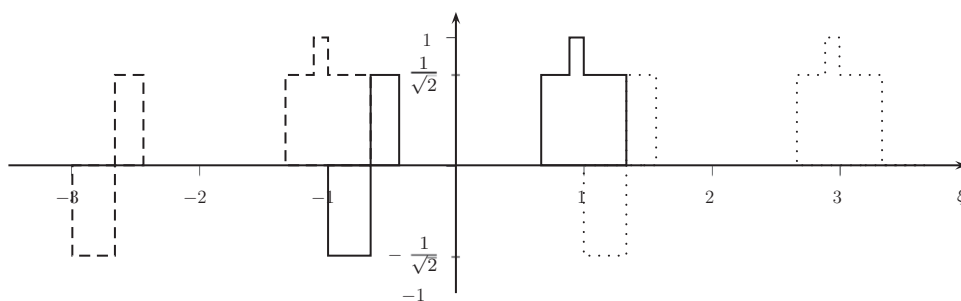
FIGURE 2. Graph of \hat{\psi}(\frac{3}{2}(\xi + 2)) (dashed), \hat{\psi}(\frac{3}{2}\xi) (solid), and \hat{\psi}(\frac{3}{2}(\xi - 2)) (dotted).
