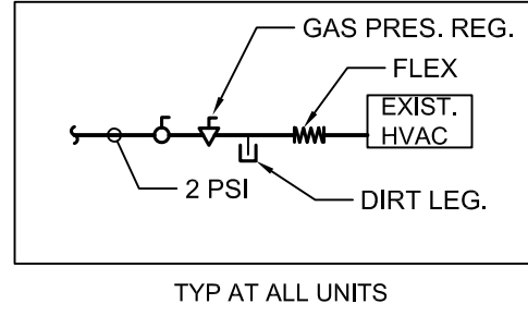
DETAIL WH-1 NTS
