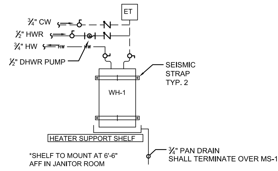
DETAIL WH-1 NTS
