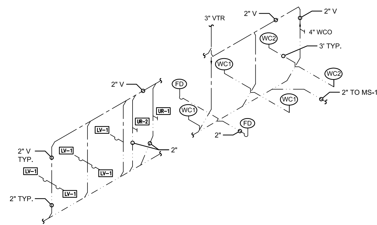
NORTH RESTROOM DWV ISOMETRIC NTS
