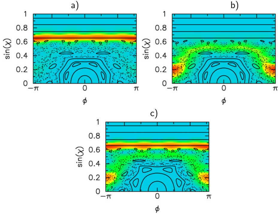
Figure 2: The projection \rho_{SOS} of the Husimi function onto the Poincaré surface section, superimposed with classical trajectories to indicate the extent of regular and chaotic regions. The uncertainty in \phi is 0.5 radians; \delta/R = 0.135 in a) and b), with a) showing the phase space density of the WG mode and b) that of the broad resonance. In c), \rho_{SOS} is shown for the WG state at \delta/R = 0.139 .
