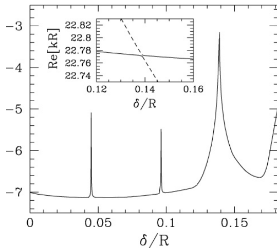
Figure 1: The width of the whispering gallery mode (2,30) as a function of the eccentricity \delta/R . Inset: Positions of the WG mode (2,30) (solid line) and the closest broad resonance (dashed line).
