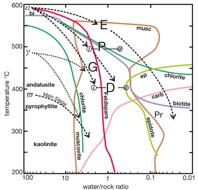
FIG. 11. Mineral stability relative to temperature and water/rock reaction ratio, as in Figure 8, but simplified to show fluid reaction trajectories and alteration mineral assemblages observed in Butte and other porphyry copper deposits. Letters E, P, G, D, and Pr refer to EDM, PGS, GS, DGS, and propylitic alteration, respectively, as described in Table 1 and in the text. The circled "i" and "o" tied by horizontal lines to "P" and "D" refer to the mineral assemblages of the inner (i) and outer (o) zones of alteration envelopes that are otherwise designated as PGS and DGS. Notice that the inner envelopes connected to PGS and DGS alteration are the same assemblage as in GS, consisting of quartz, chlorite, and muscovite, but lacking feldspars. " \alpha " refers to magmatic fluid as observed in B35 inclusions, which reacts and cools along trajectories shown by dashed curves to generate the potassic vein series described in the text. " \gamma " refers to fluid observed in B60 inclusions interpreted as a cooled and depressurized \alpha fluid responsible for generating the GS veins that are abundant in the center of the district (Figs. 1, 3). " \omega " refers to a further cooled and depressurized fluid responsible for main stage vein mineralization.
