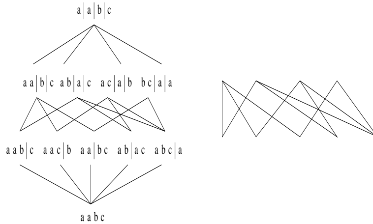
FIGURE 4. \Pi_4/S_2 \times S_1 \times S_1 and its (1-dimensional) order complex
