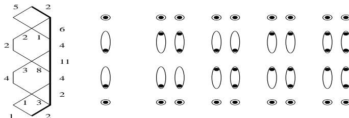
FIGURE 3. A matching example
