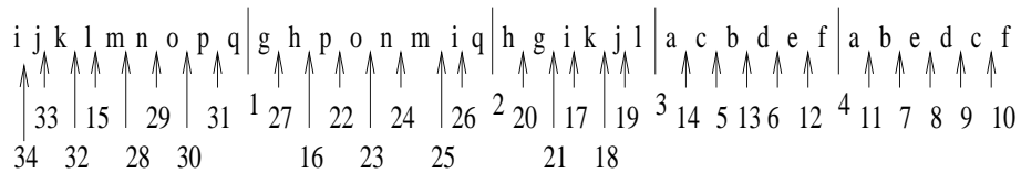
FIGURE 10. A saturated chain e\sigma to be paired with \rho
