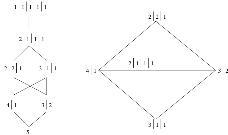
FIGURE 5. \Pi_5/S_5 and its (2-dimensional) order complex \Delta(\Pi_5/S_5)
