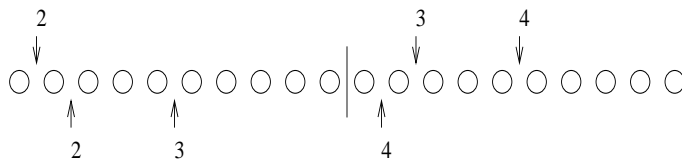
FIGURE 6. An example of type 1
