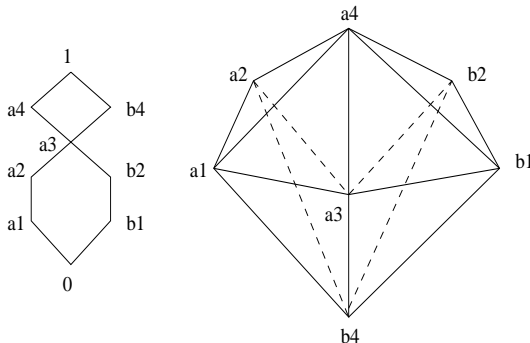
FIGURE 2. A poset and its order complex
