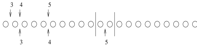
FIGURE 8. An example of type 3
