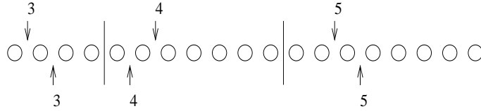
FIGURE 7. An example of type 2
