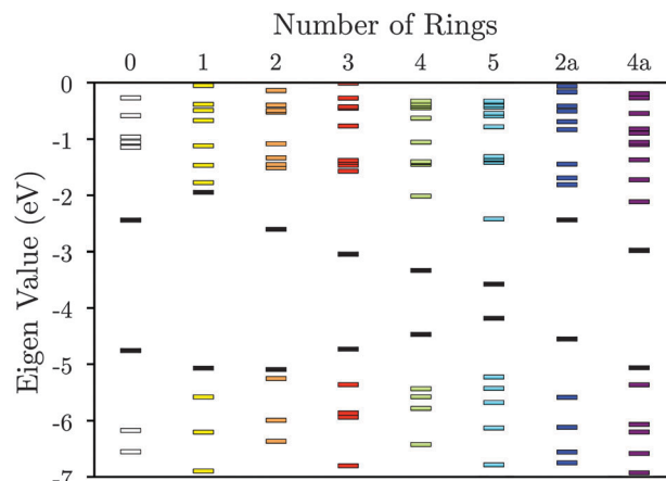
Fig. 3 Molecular orbital energies for the tetrathiol ligands of Fig. 2. The black lines denote HOMOs and LUMOs. The vacuum level is set to 0 eV.
