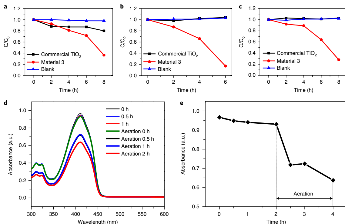
Fig. 6 | Photochemical data for material 3. a–c , Photocatalytic degradation of three dyes, alizarin red S (ARS) ( a ), methylene blue (MB) ( b ) and rhodamine B (RhB) ( c ), under red ( \sim 630 nm) LED light conditions. In each case, material 3 was found to catalyse the photodegradation of the dye at substantially faster rates than commercial TiO 2 . d , UV-vis spectrum that depicts the progression of the consumption of 1,3-diphenylisobenzofuran (DPBF) in the presence of material 3 and irradiation with red ( \sim 630 nm) LED lights. DPBF is a sensitive fluorescent probe for ROS, and a decrease in its absorbance at 410 nm is indicative of the production of ROS. Aeration of the reaction mixture leads to increased rates of consumption of DPBF, consistent with ROS production. e , The chart shows the rate of consumption of DPBF.
